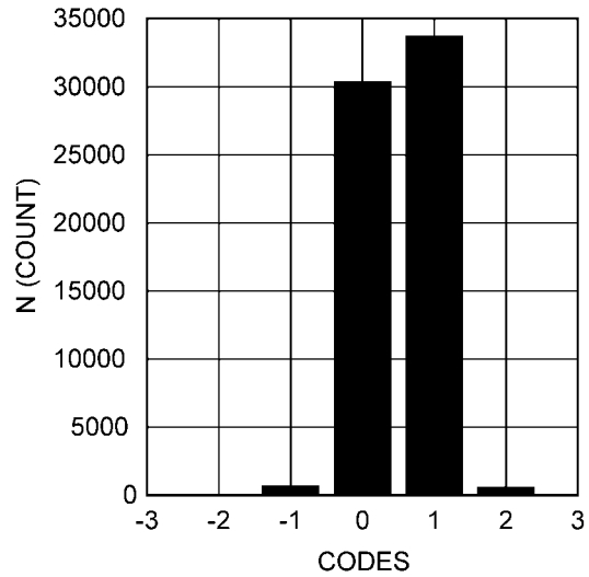
FIGURE 14. Noise Histogram at Code Transition
