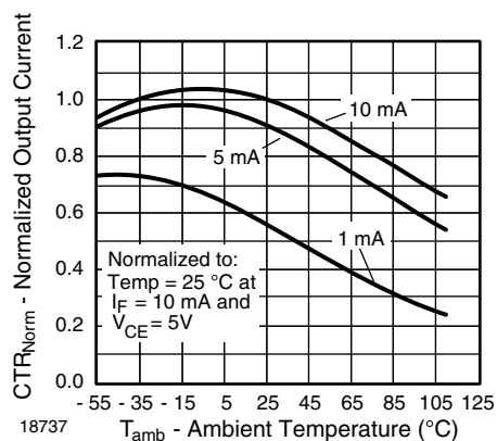
Fig. 9 - Normalized CTR vs. Temperature
