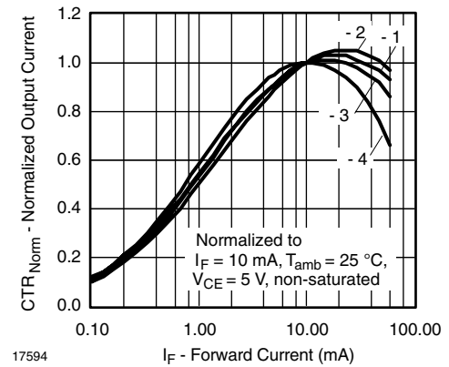
Fig. 10 - Normalized CTR vs. Forward Current
