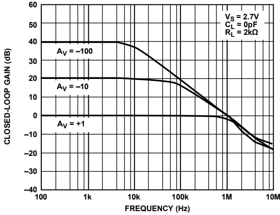
Figure 19. Closed-Loop Gain vs. Frequency at 2.7 V
