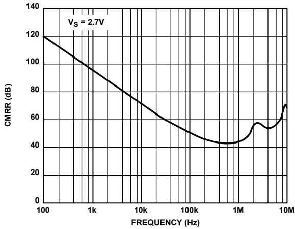
Figure 32. CMRR vs. Frequency at 2.7 V
