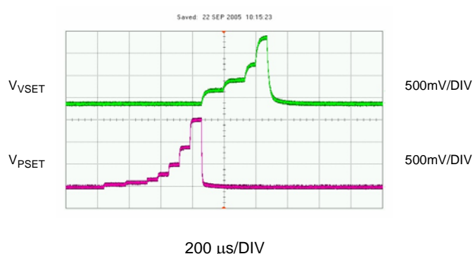
Figure 12: VSET = 2.5V and PSET = -5%
