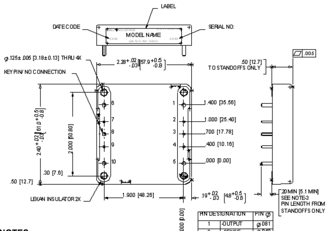
Figure 1: Mechanical Dimensions
