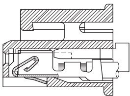
TERMINAL ASSEMBLY DRAWING
