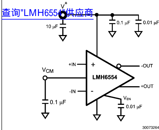
FIGURE 9. Single Supply Bypassing Capacitors
