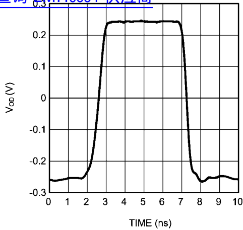
0.5 V PP Pulse Response Single Ended Input 查询"LMH6554"供应商
