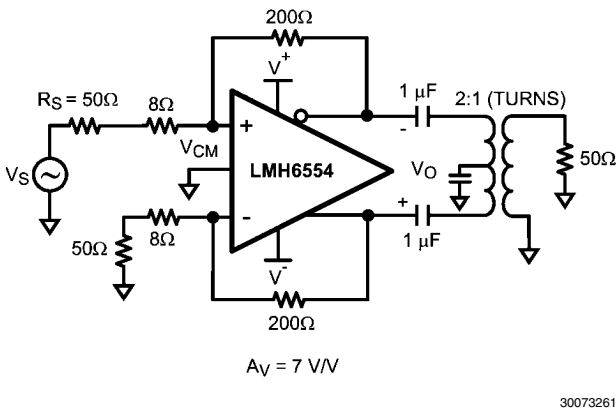
FIGURE 6. Noise Figure Circuit Configuration
