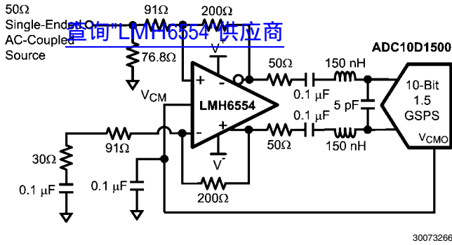
FIGURE 5. Driving a 10-bit Gigasample ADC
