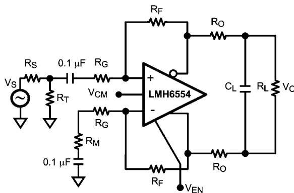
FIGURE 3. AC Coupled for Single Supply Operation
