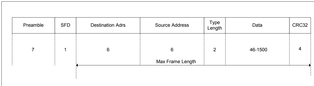
Figure 8-7. IEEE 802.3 Ethernet Frame
