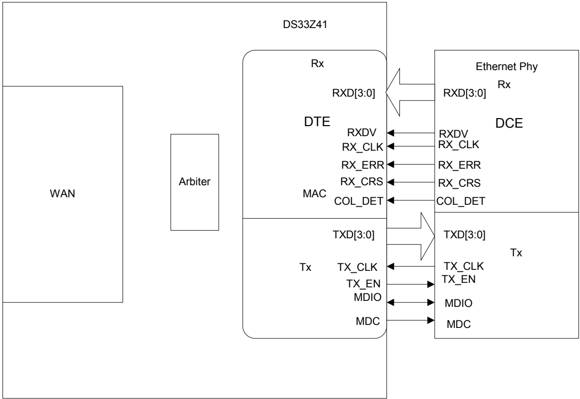
Figure 8-8. Configured as DTE Connected to an Ethernet PHY in MII Mode
