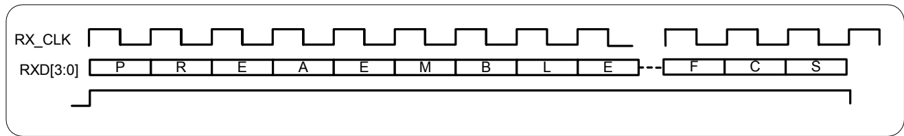
Figure 10-3. MII Receive Functional Timing
