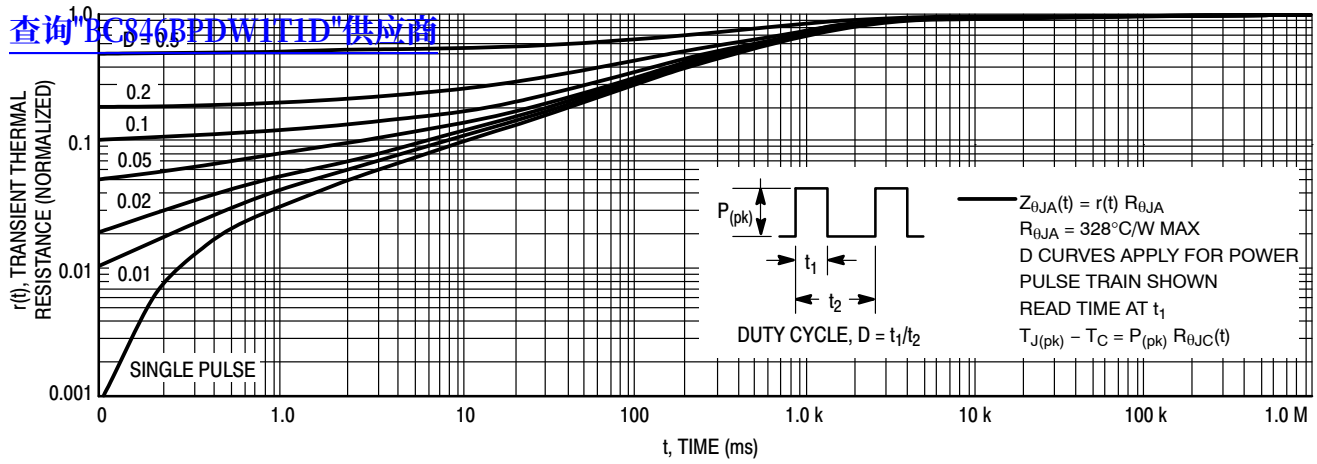
Figure 49. Thermal Response
