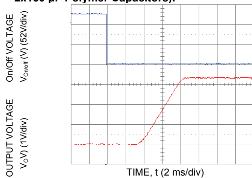
Figure 14. Typical Start-Up Using Remote On/Off ( V_{in} = 5\text{ Vdc} , V_o = 3.3\text{ Vdc} , I_o = 5\text{ A} ).
