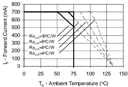
Figure 5a. Maximum Forward Current vs. Ambient Temperature. Derating based on T_{JMAX} = 135^\circ\text{C} for White, Green, Cyan and Blue 6-Up Ring.
