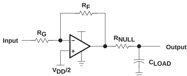
Figure 29. Driving a Capacitive Load
