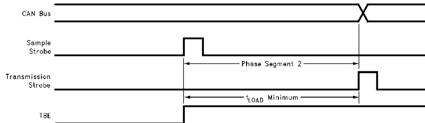
FIGURE 17. TBE Timing
