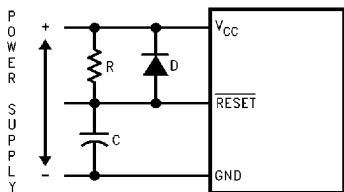
FIGURE 6. Recommended Reset Circuit
