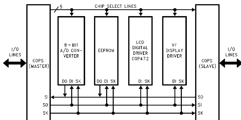
FIGURE 34. MICROWIRE/PLUS Application
