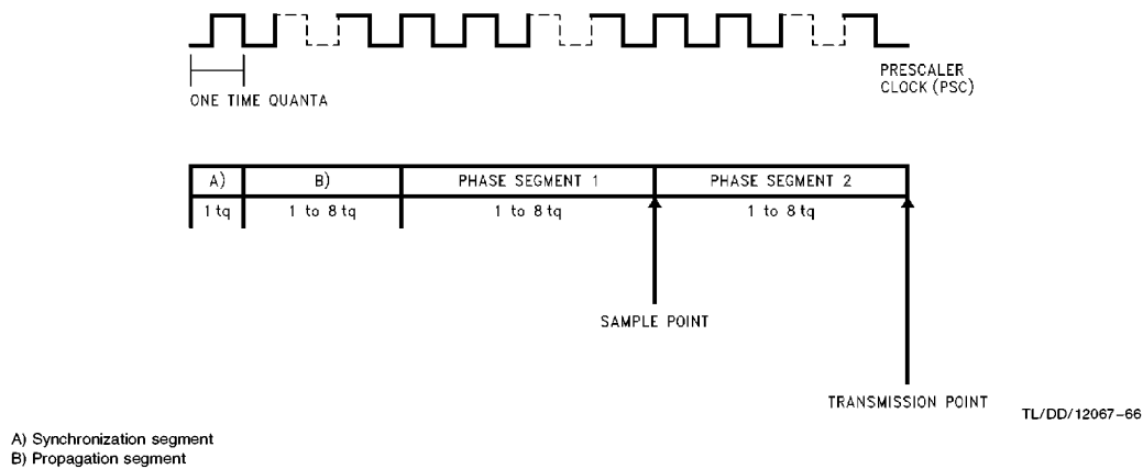
FIGURE 29. Bit Timing
