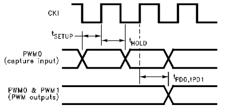
FIGURE 4. PWM/CAPTURE Timer Input/Output Timing Diagram
