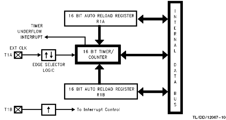
FIGURE 10. Timer 1 in External Event Counter Mode
