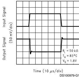
Small Signal Inverting Response
