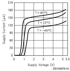
Supply Current vs. Supply Voltage (LMV921)
