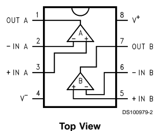
8-Pin MSOP/SOIC
