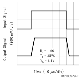
*Large Signal Non-Inverting Response
