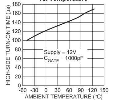
High-Side Turn-On Time vs. Temperature
