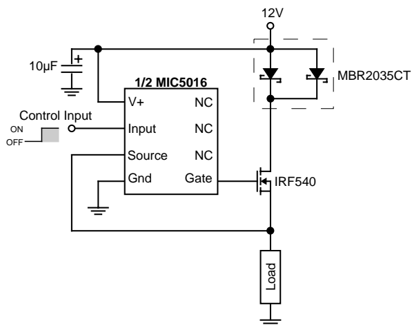
Figure 12: High Side Driver Wlth Load Protection
