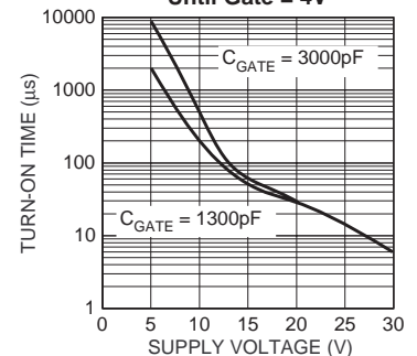
Low-Side Turn-On Time Until Gate = 4V
