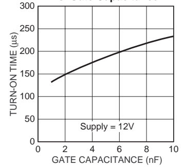
High-Side Turn-On Time vs. Gate Capacitance
