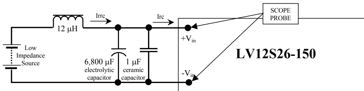
Figure 9: Ripple Current Setup
