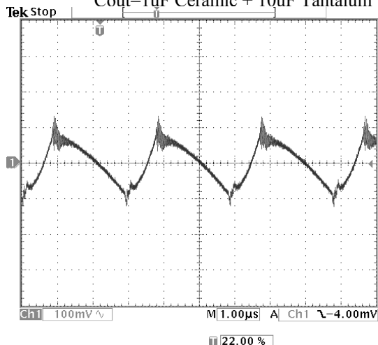
Photo 11: Output Voltage Ripple (Spike) V_{in}=24V , I_{out} = 5.8A C_{out}=1\mu F Ceramic + 10\mu F Tantalum
