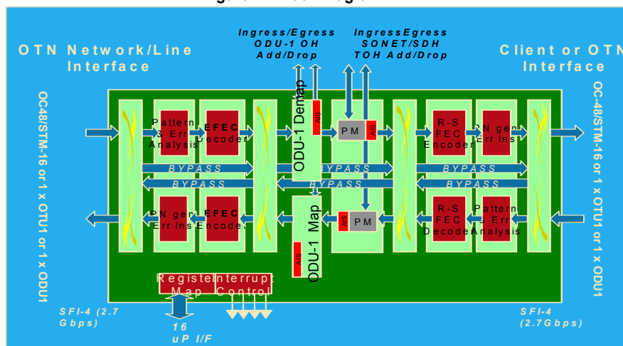
Figure 1: Block Diagram
