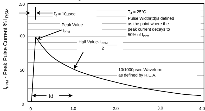
Fig.3 - Pulse Waveform
