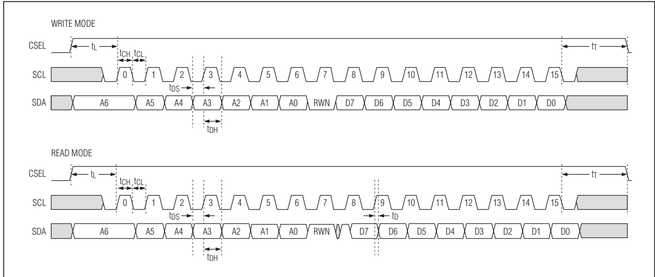
Figure 5. Timing for the 3-Wire Digital Interface
