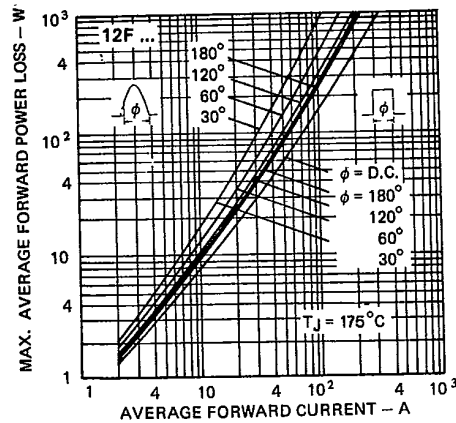
Fig. 9 - Maximum Forward Power Loss Vs. Average Forward Current, 12F Series
