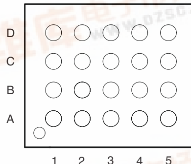
TERMINAL ASSIGNMENTS
