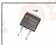
PG-TO263-3-2
