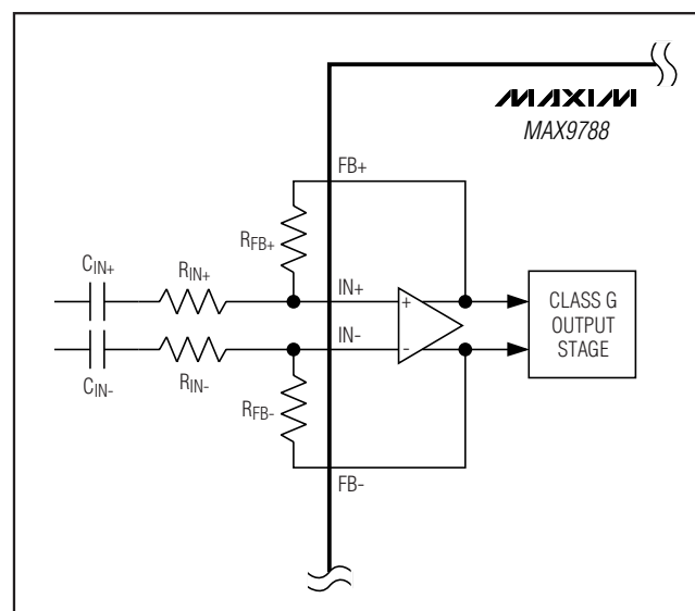
Figure 2. Gain Setting
