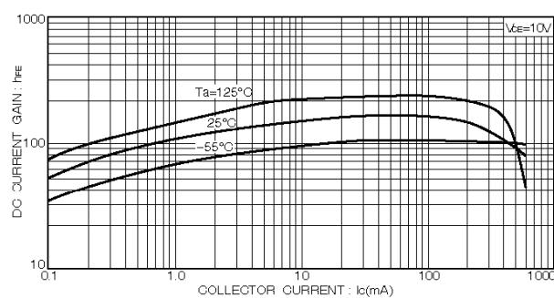
Fig.4 DC current gain vs. collector current(II)
