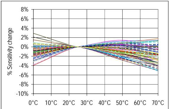
Graph 13. Examples of A OUTX Sensitivity change over temperature
