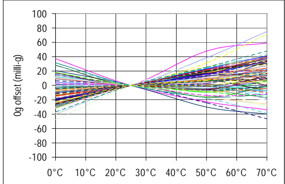
Graph 11. Examples of A OUTX 0g offset vs. temperature
