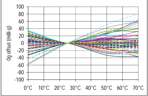
Graph 12. Examples of A OUTY 0g offset vs. temperature
