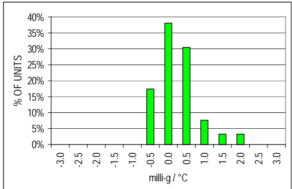
Graph 10. Distribution of A OUTY 0g offset over temperature
