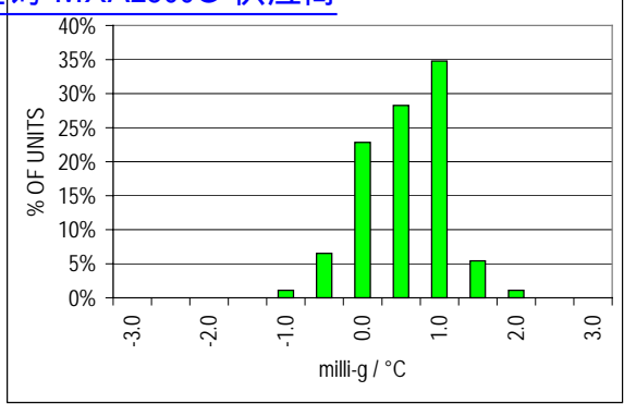
Graph 9. Distribution of A OUTX 0g offset over temperature
