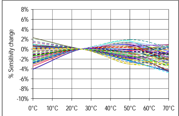
Graph 14. Examples of A OUTY Sensitivity change over temperature
