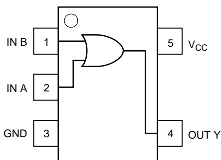
Figure 1. Pinout
