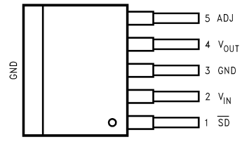
Top View TO263-5 Package
