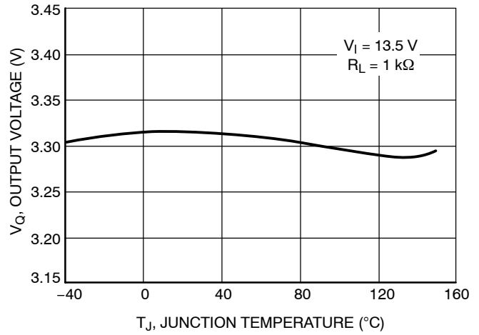
Figure 29. Output Voltage V_O vs. Junction Temperature T_J , 3.3 V Version
