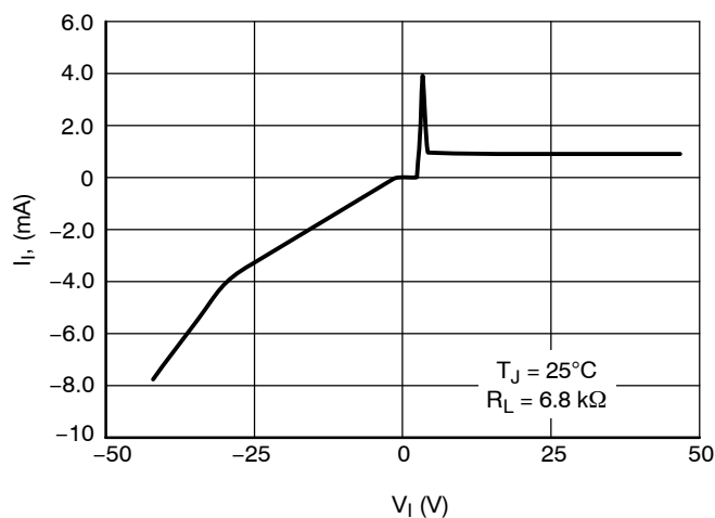
Figure 24. Input Current I_I vs. Input Voltage V_I , 5.0 V Version
