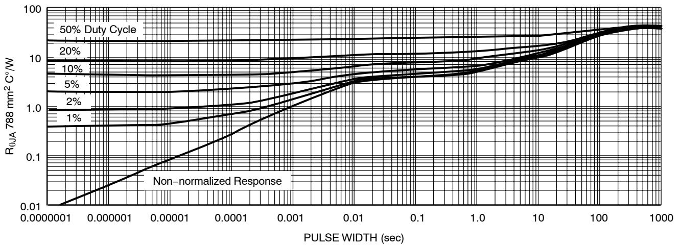
Figure 56. Duty Cycle for 1" Spreader Boards, D²PAK 5-Lead
