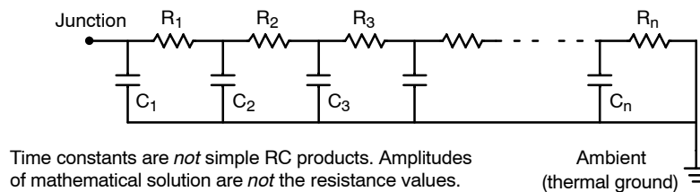
Figure 49. Grounded Capacitor Thermal Network ("Cauer" Ladder)
