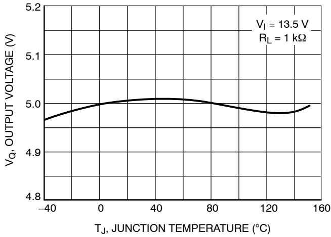
Figure 28. Output Voltage V_O vs. Junction Temperature T_J , 5.0 V Version
