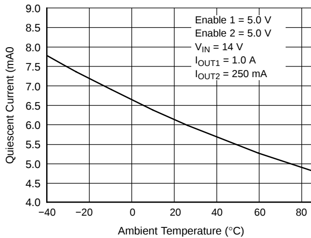
Figure 8. Quiescent Current
