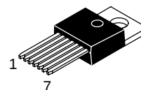
TO-220 SEVEN LEAD T SUFFIX CASE 821E
