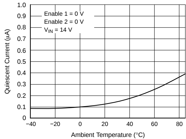
Figure 9. Quiescent Current
