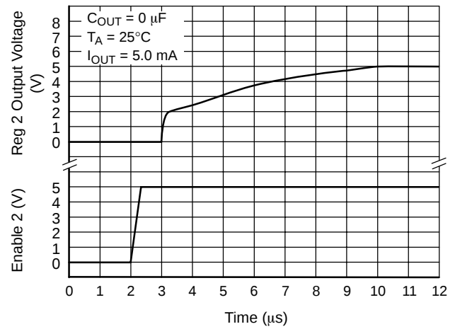
Figure 15. Regulator 2 Startup
