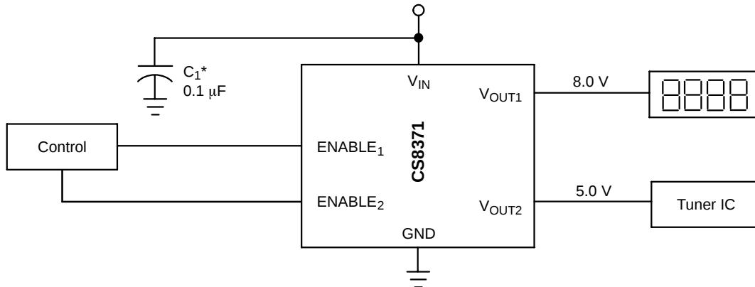
Figure 23. Applications Circuit
