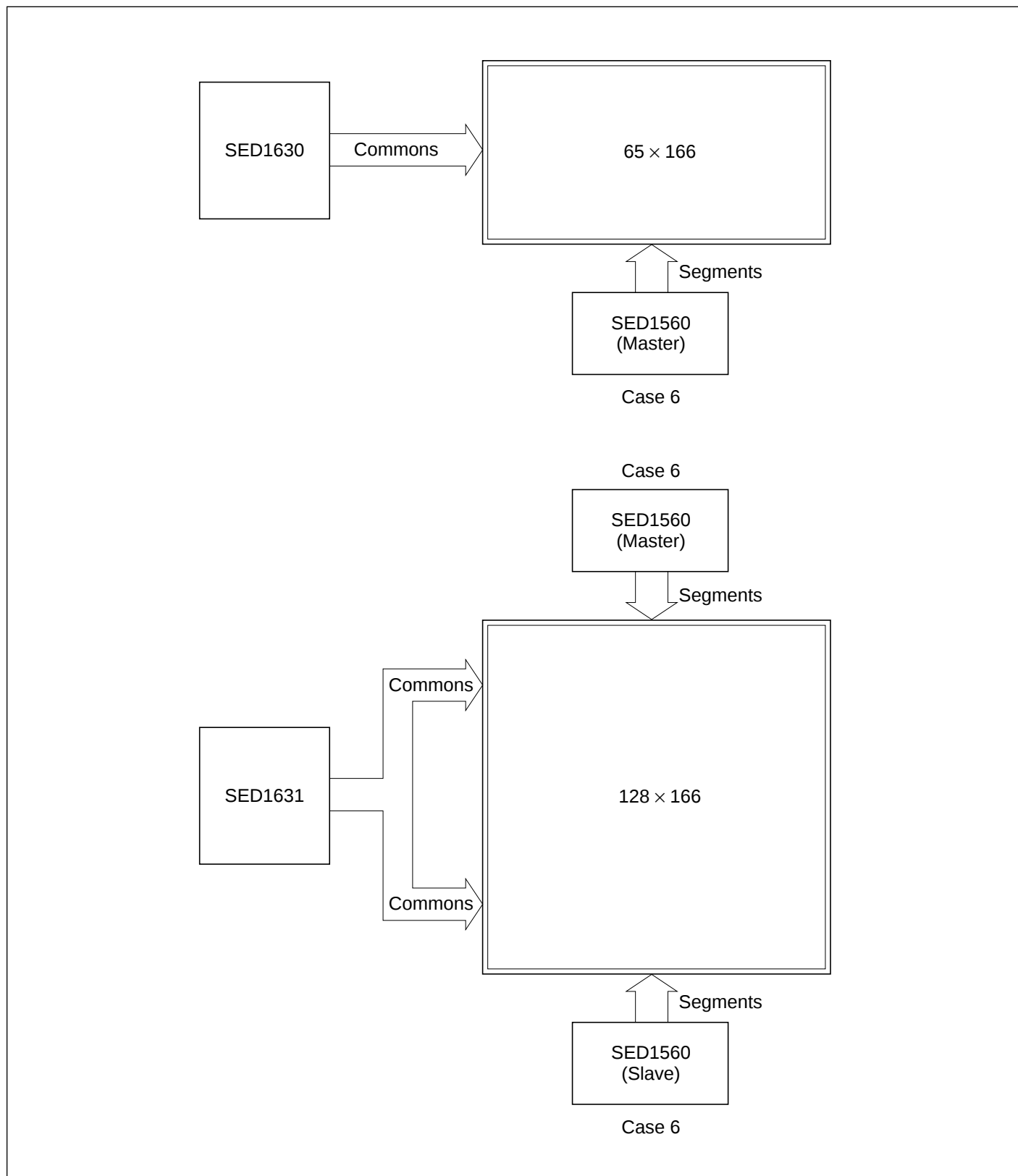
Figure 5.11 Special common driver configurations
