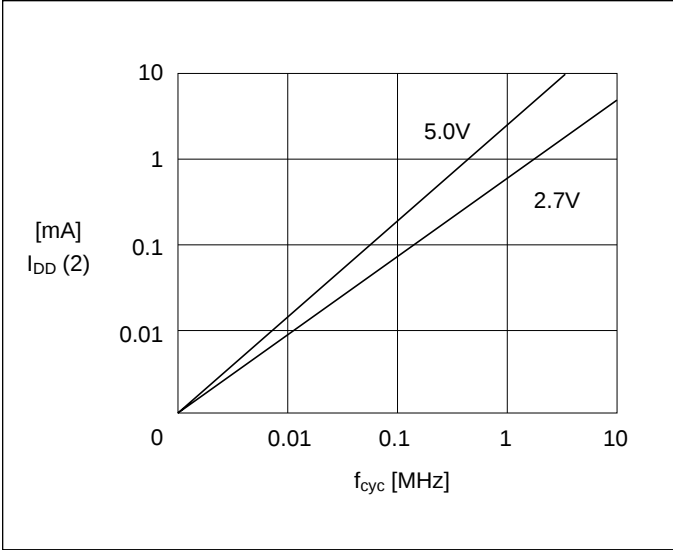
Figure 3.4 Power consumption during CPU access cycle (IDD [2])
