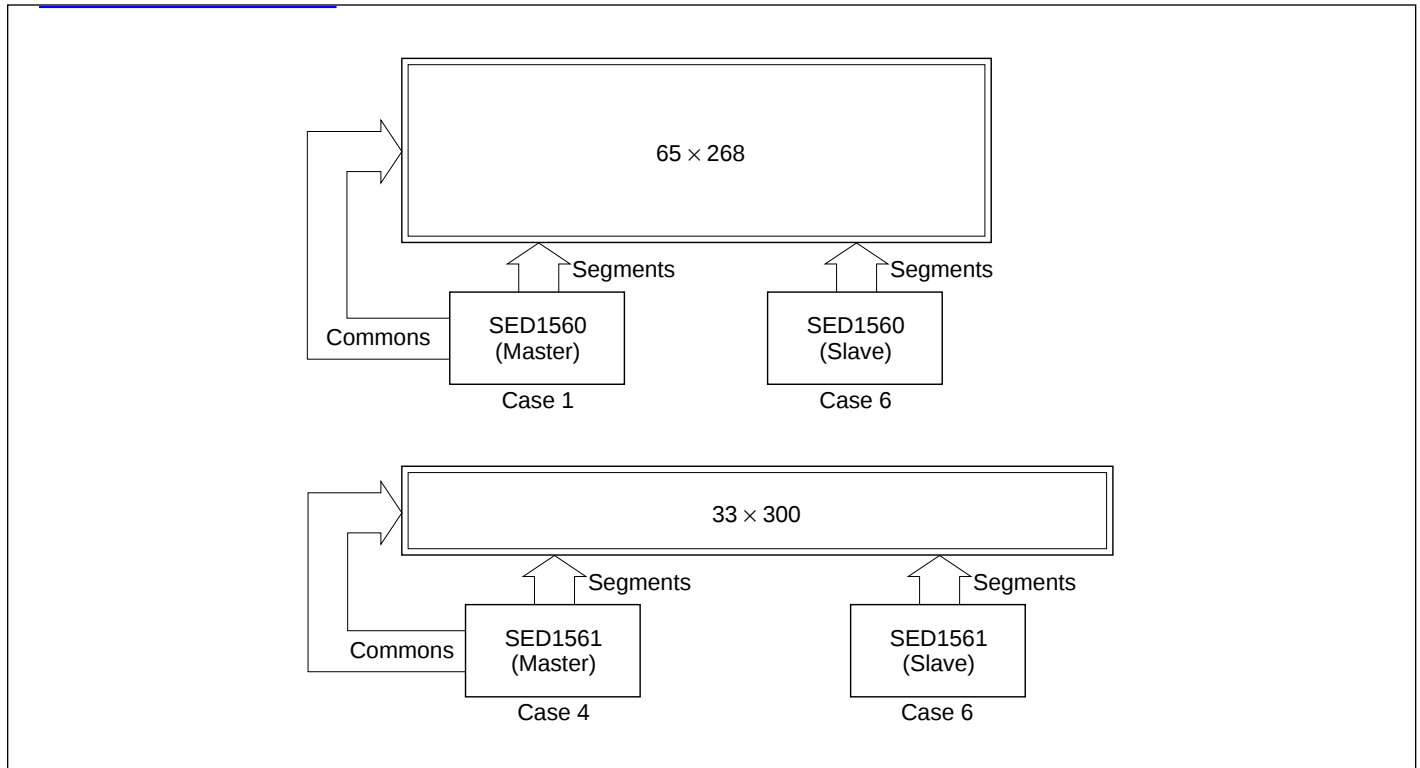
Figure 5.10 Multiple-chip combinations
