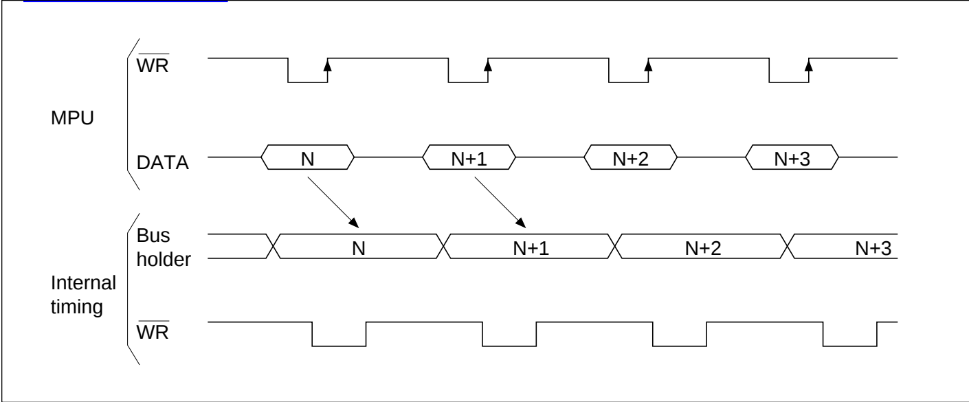
Figure 4.2 Write timing
