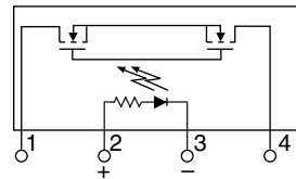
CPC1218Y Pinout
