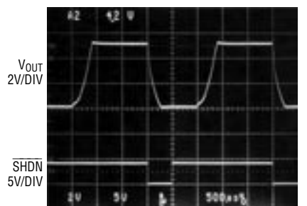
V_{\text{OUT}} Soft-Start
