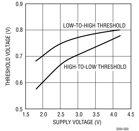
SHDN Threshold Voltage vs Supply Voltage
