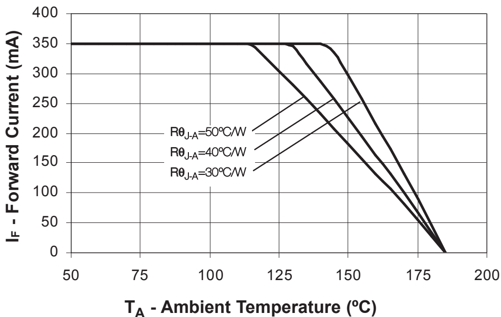
Figure 20: Maximum forward current vs. ambient temperature, based on T_{JMAX} = 185^{\circ}C .
