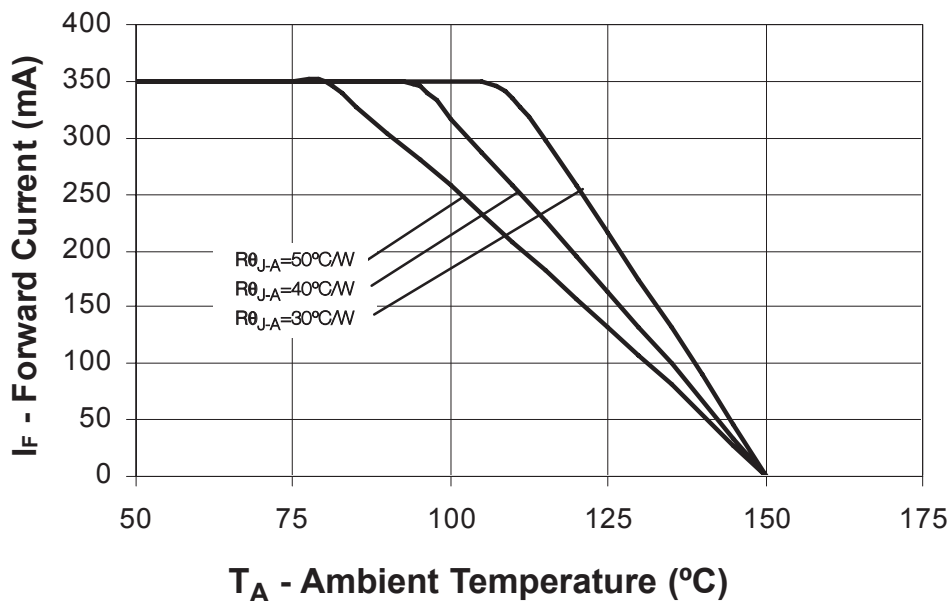
Figure 19: Maximum forward current vs. ambient temperature, based on T_{JMAX} = 150^{\circ}C .
