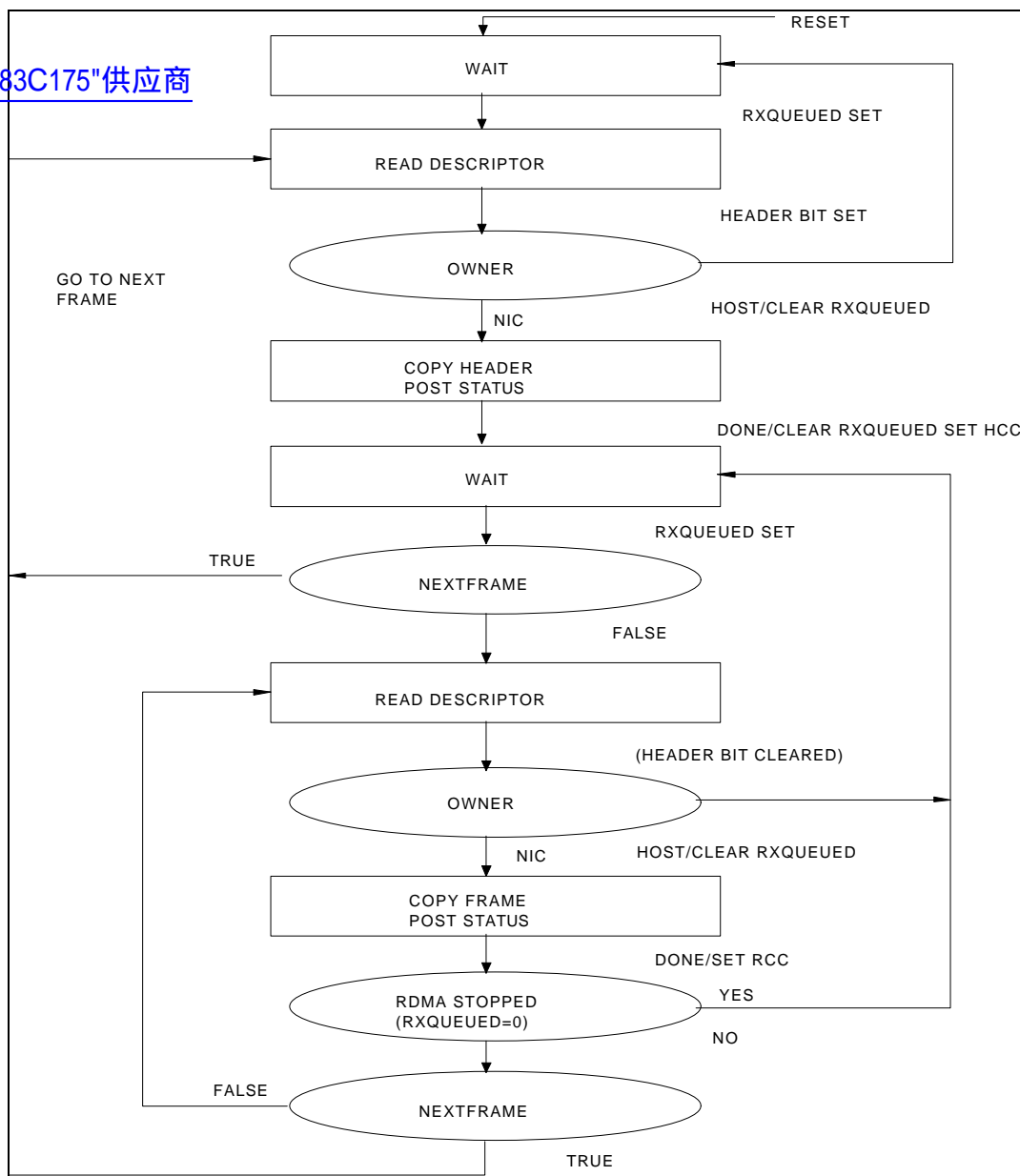
FIGURE 4 - RECEIVE LOCKAHEAD BUFFERING FLOW
