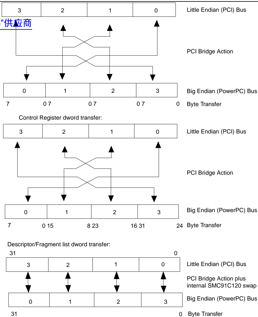
FIGURE 5 - LITTLE ENDIAN/BIG ENDIAN BYTE TRANSFER
