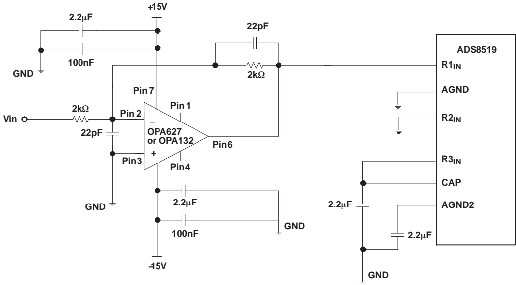
Figure 31. Typical Driving Circuitry ( \pm 10\text{V} , No Trim)
