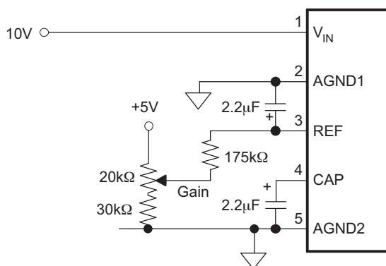
(a) 10V With Hardware Trim
