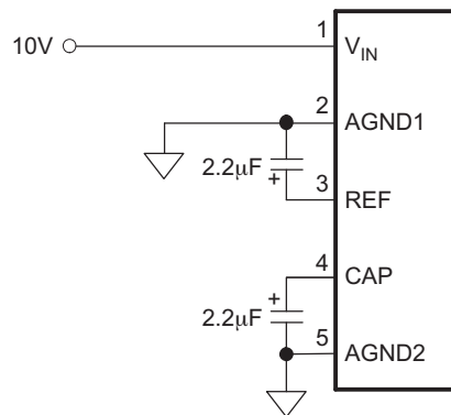
(b) 10V Without Hardware Trim
