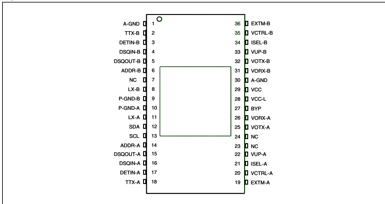
Figure 3. Pin connections
