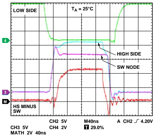
Figure 59. Output Drivers and SW Node Waveforms
