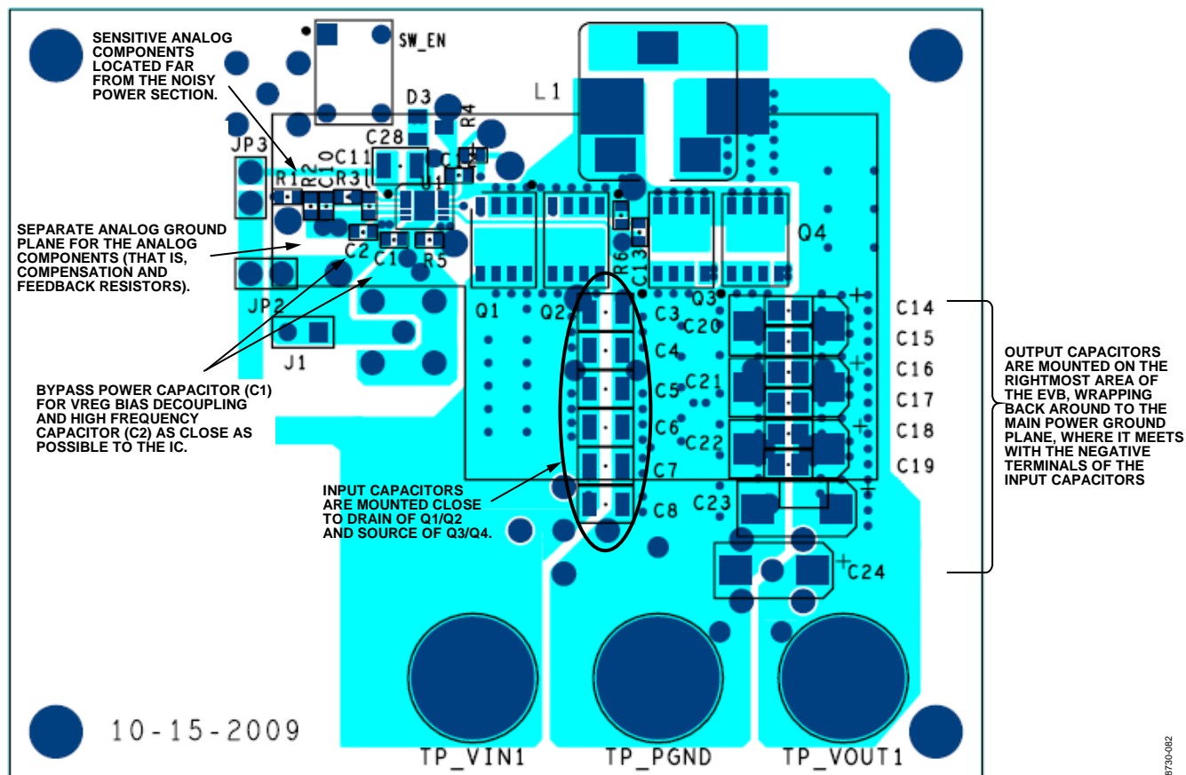
Figure 86. Overall Layout of the ADP1870 High Current Evaluation Board
