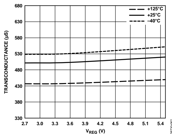
Figure 63. Transconductance ( G_m ) vs. V_{REG}
