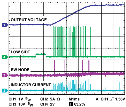
Figure 58. Soft Start and RES Detect Waveform
