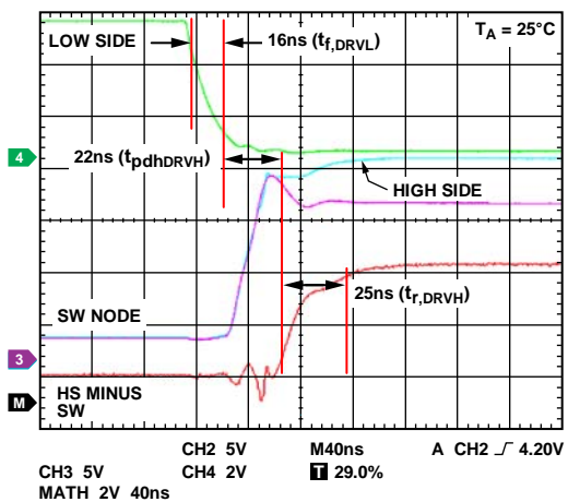
Figure 60. Upper-Side Driver Rising and Lower-Side Falling Edge Waveforms ( C_{IN} = 4.3 \text{ nF} (Upper-/Lower-Side MOSFET), Q_{TOTAL} = 27 \text{ nC} ( V_{GS} = 4.4 \text{ V} (Q1), V_{GS} = 5 \text{ V} (Q3))
