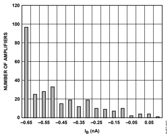
Figure 7. Input Bias Current, V_{SY} = \pm 15\text{ V}
