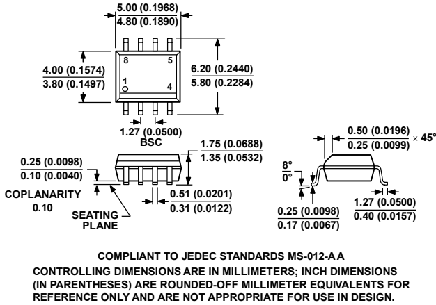
Figure 27. 8-Lead Standard Small Outline Package [SOIC_N] Narrow Body (R-8) Dimensions shown in millimeters and (inches)
