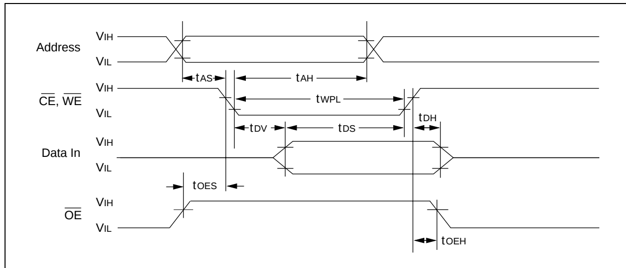
FIGURE 1-2: PROGRAMMING WAVEFORMS
