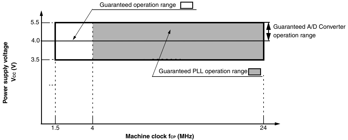
Guaranteed operation range of MB90860E series
