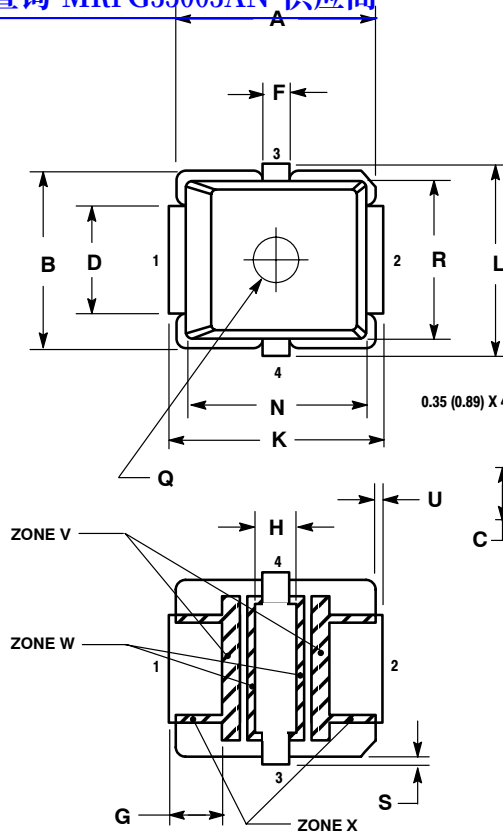
VIEW Y-Y
