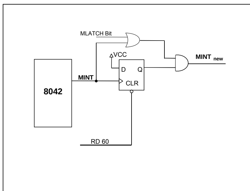
FIGURE 6 – MOUSE LATCH
