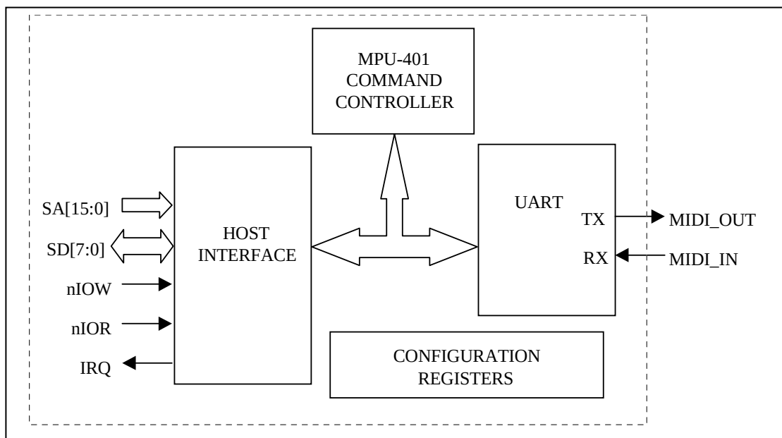
FIGURE 2 - MPU-401 MIDI INTERFACE
