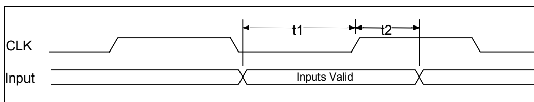
FIGURE 11 – INPUT TIMING MEASUREMENT CONDITIONS, LPC SIGNALS
