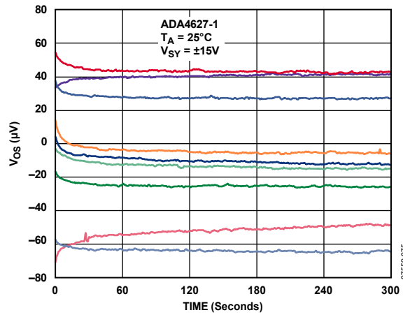
Figure 22. Input Offset Voltage vs. Time
