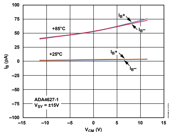
Figure 20. Input Bias Current vs. V_{CM} and Temperature
