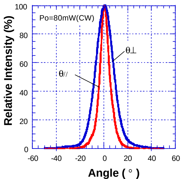
Far-Field-Patterns
