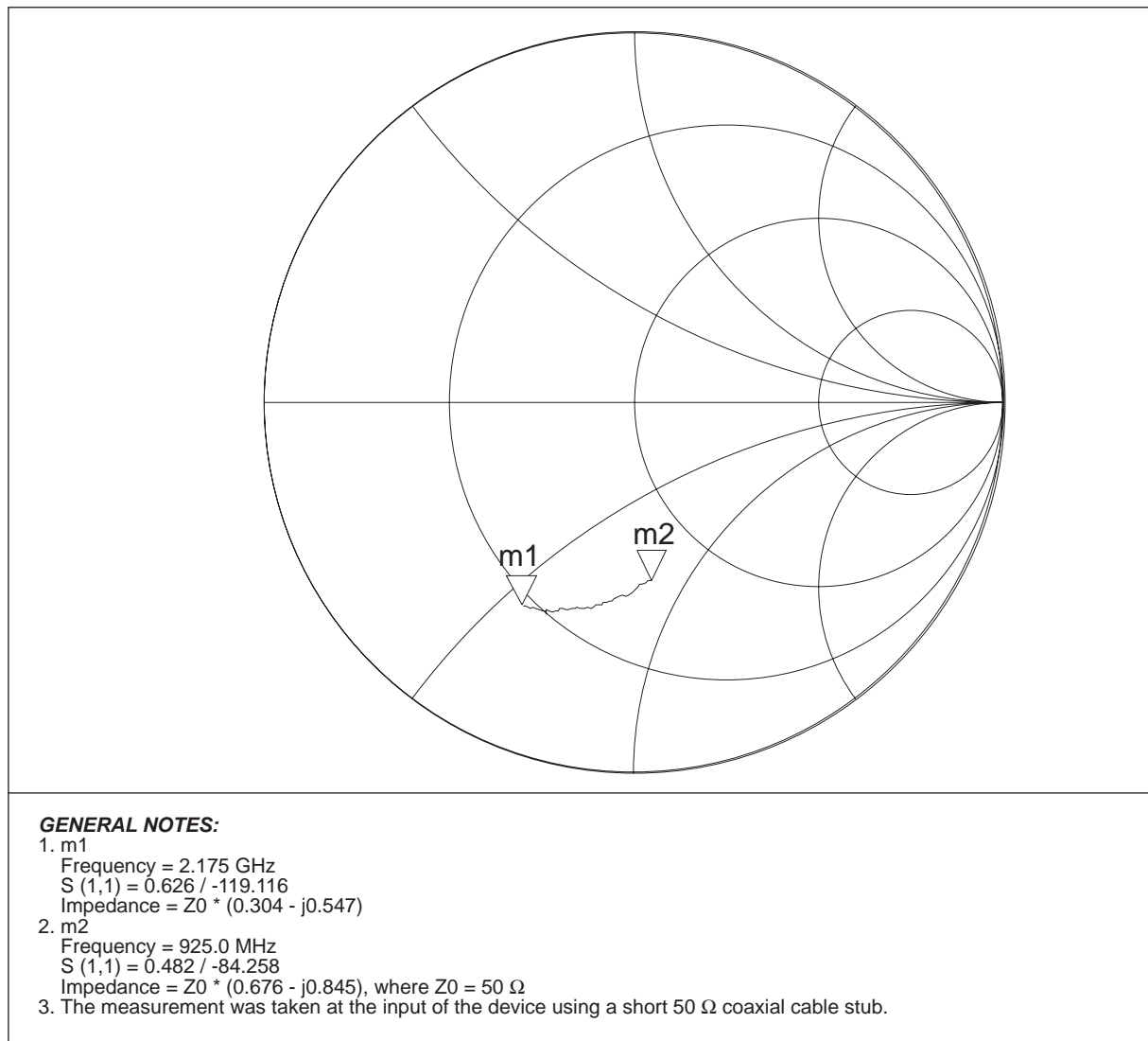
Figure 10. S11 Plot
