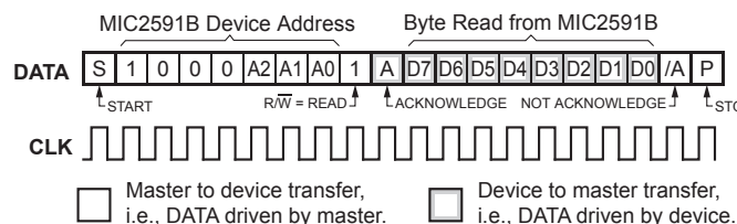
Figure 12. RECEIVE_BYTE Protocol
