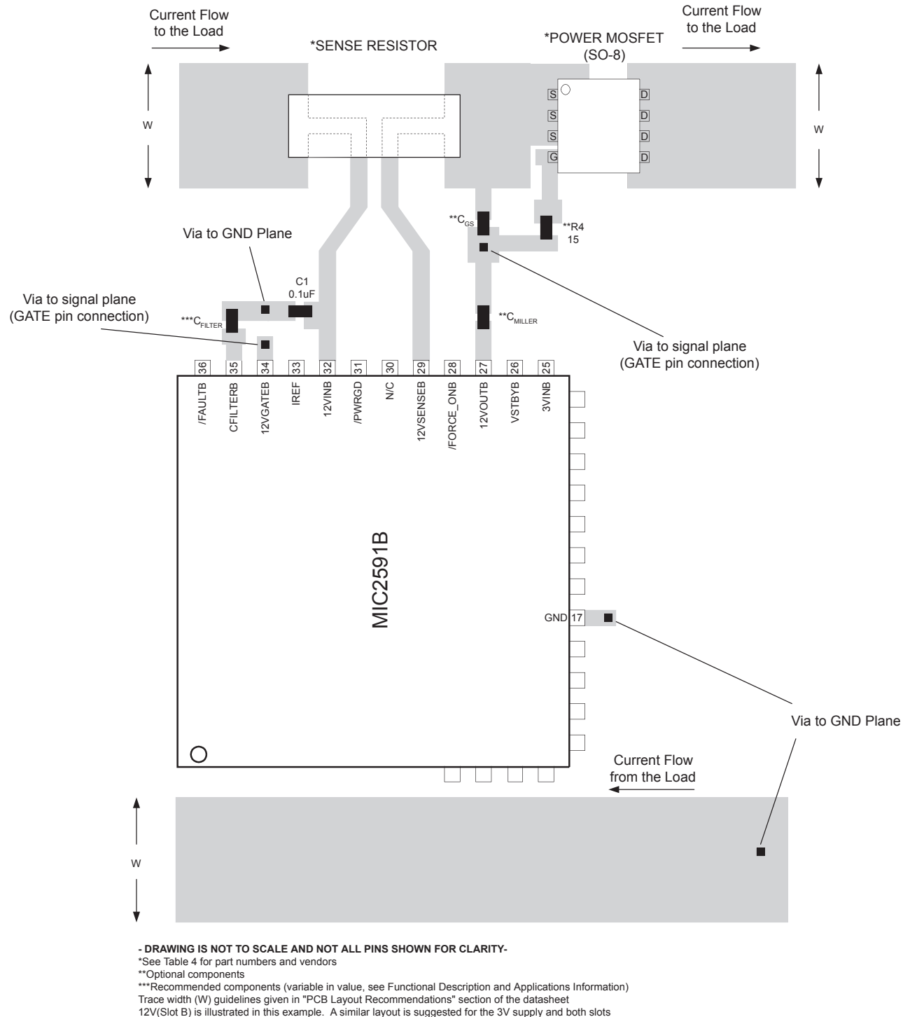
Figure 15. Suggested PCB Layout for Sense Resistor, Power MOSFET, and Capacitors
