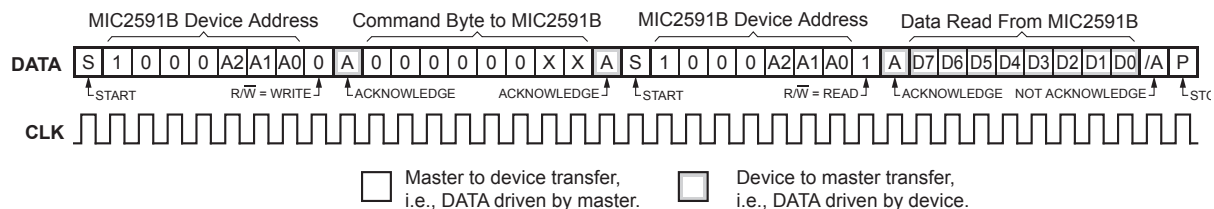
Figure 11. READ_BYTE Protocol
