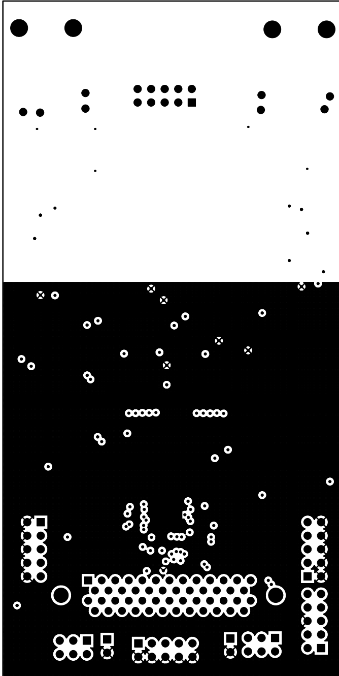
Figure 7. Si3232DC0-EVB Ground
