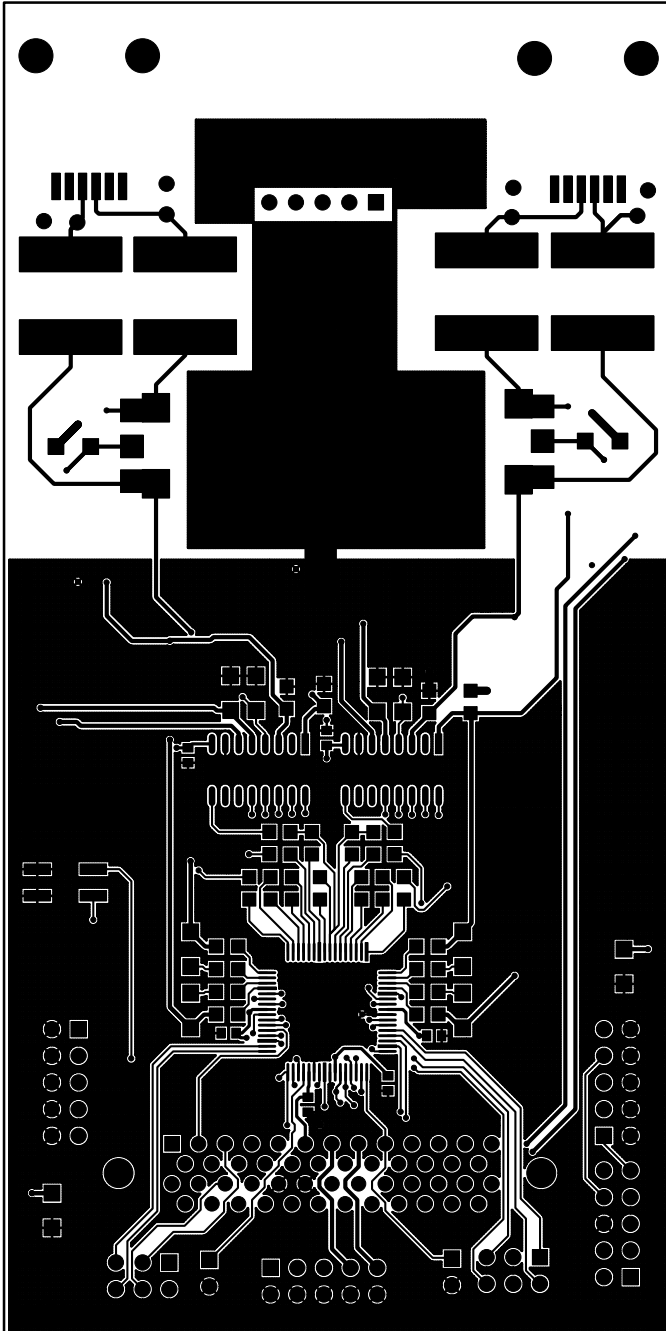
Figure 5. Si3232DC0-EVB Component Side
