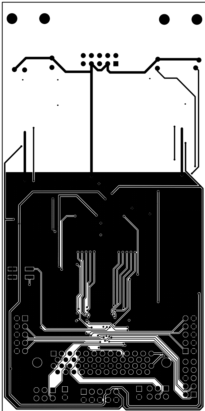
Figure 8. Si3232DC0-EVB Solder Side
