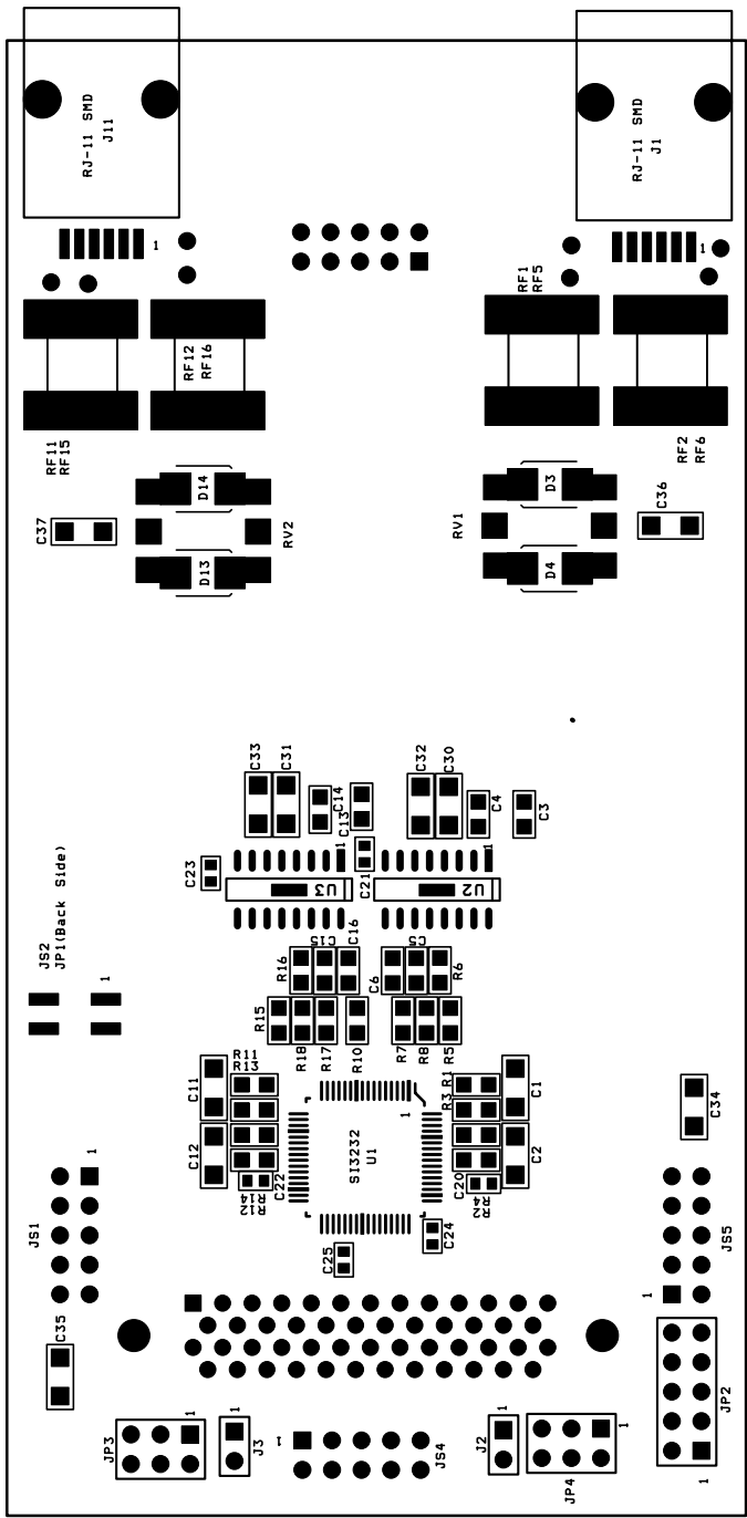
Figure 4. Si3232DC0-EVB Silkscreen
