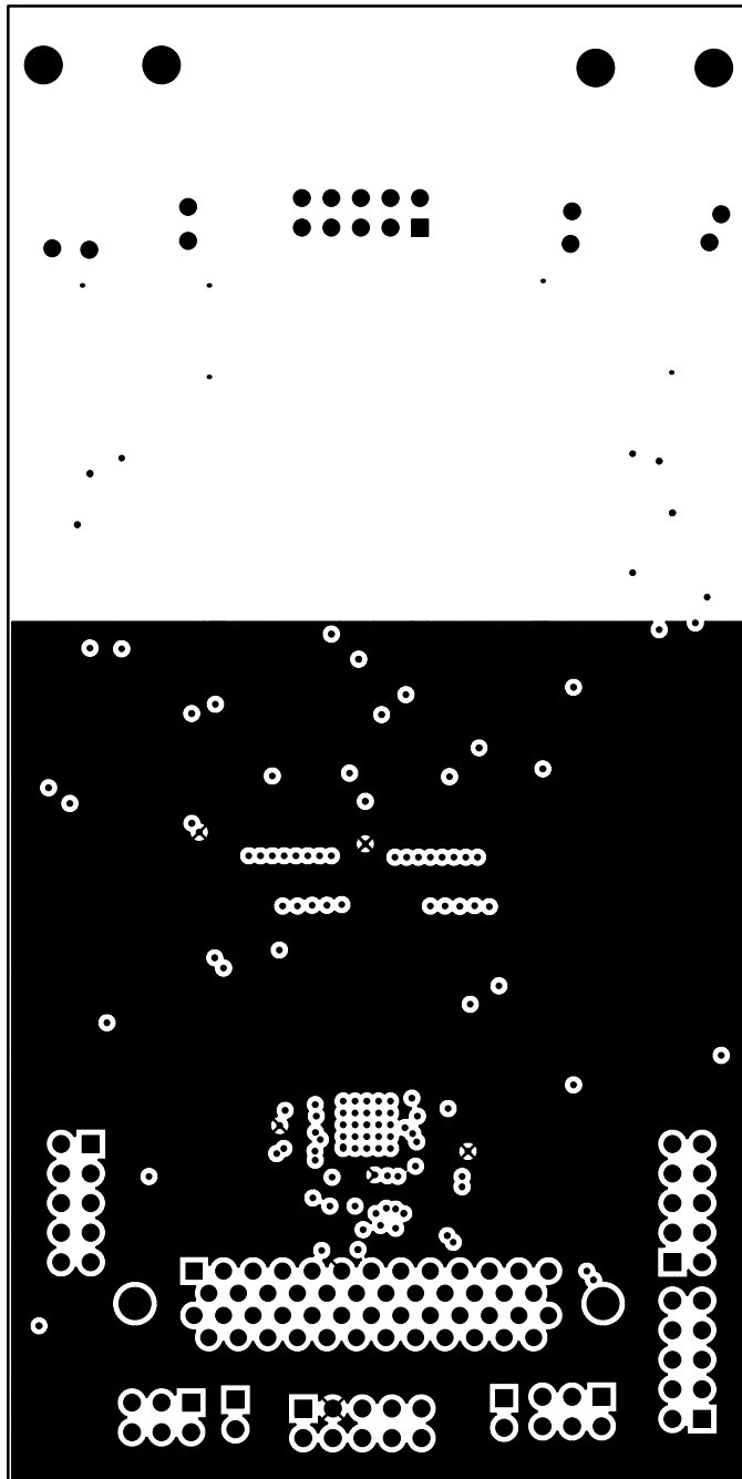
Figure 6. Si3232DC0-EVB Power
