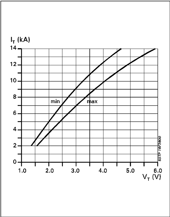
Fig. 3 On-state characteristics. T j =125°C, 10ms half sine
