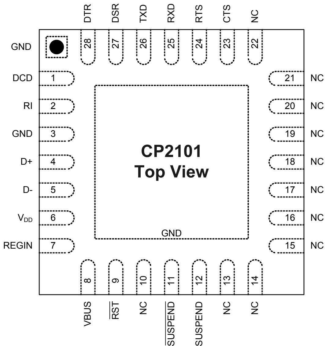
Figure 4.1. QFN-28 Pinout Diagram (Top View)
