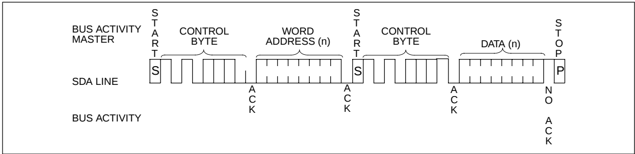
FIGURE 7-2: RANDOM READ
